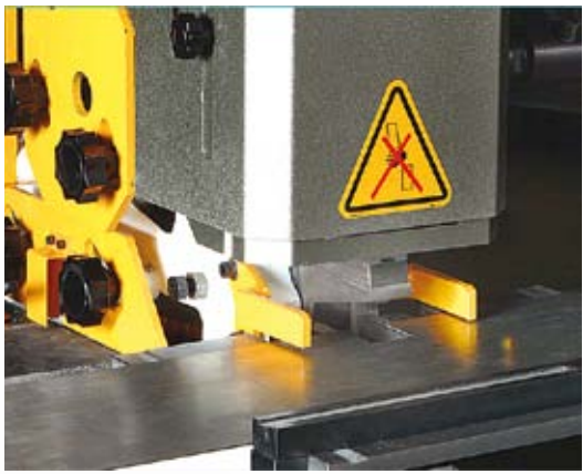
Notching Station
